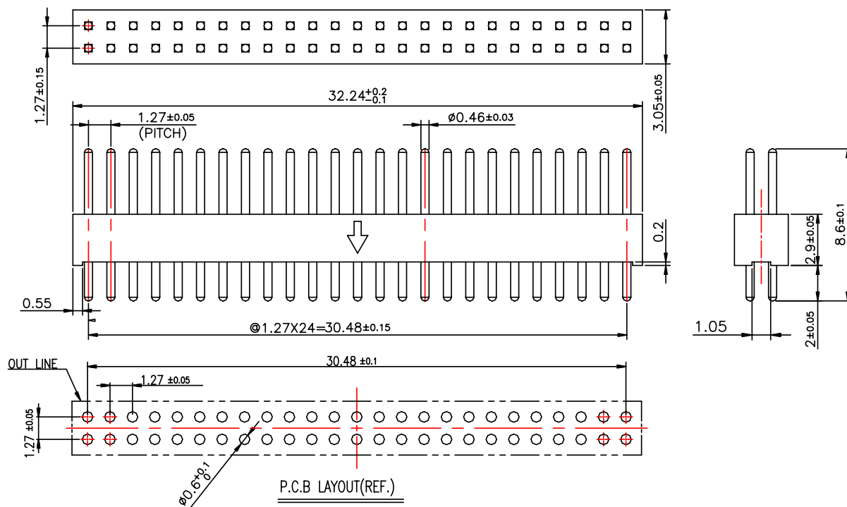
EBB-PH23-PA**T2 UNIT:mm Connection Style: Straight Plug
