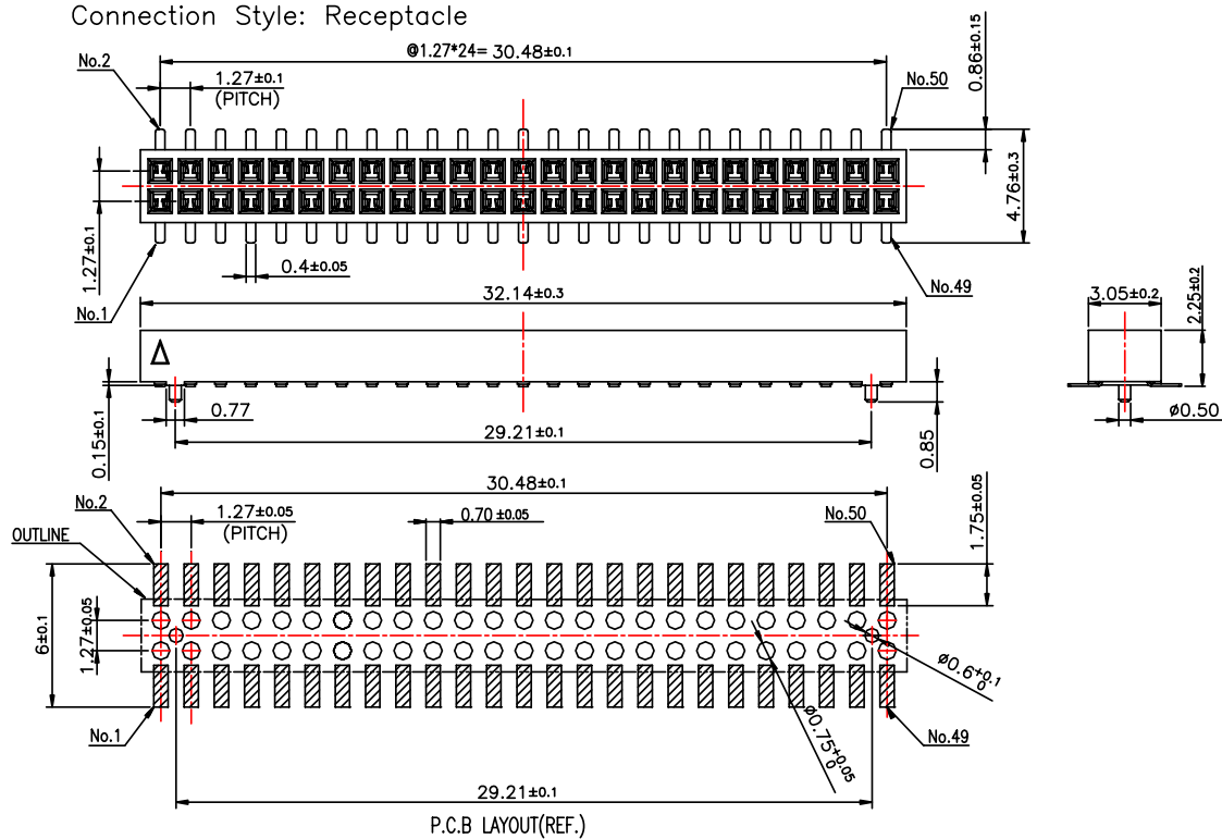
EBB-PH23-SA**V2 UNIT:mm Connection Style: Receptacle
