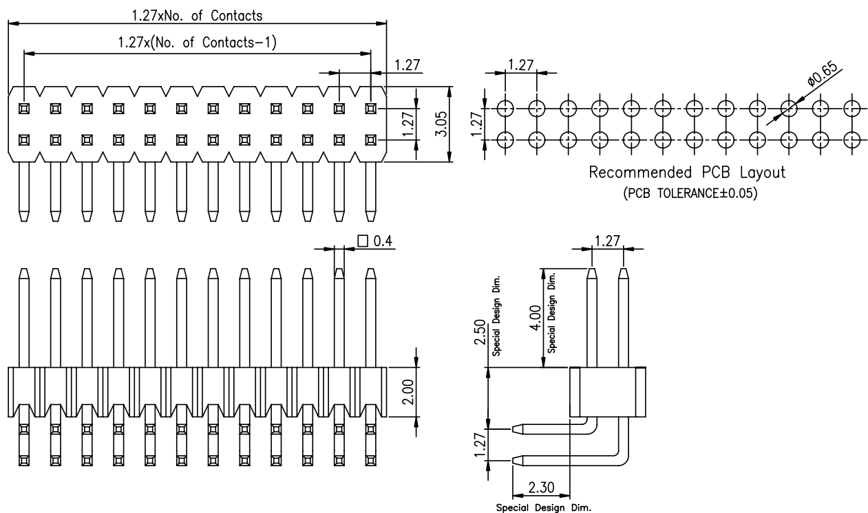
DIMENSIONS UNIT:mm EBB15-PDxxL
