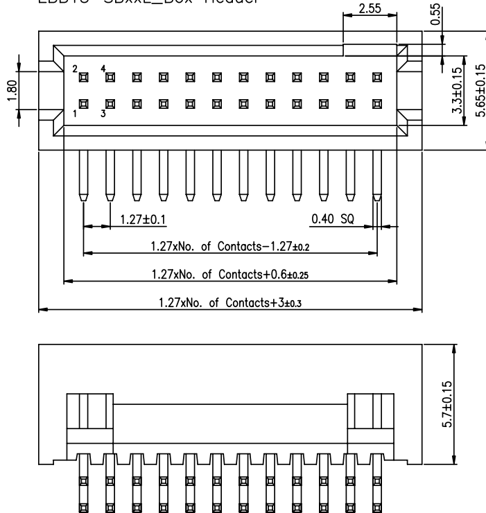
DIMENSIONS UNIT:mm EBB15-SBxxL_Box Header
