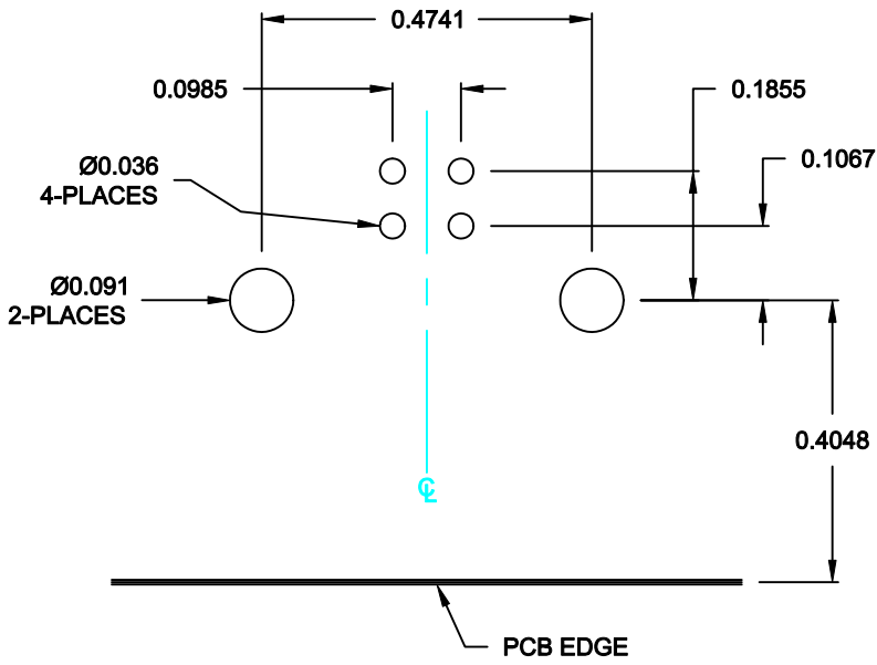
RECOMMENDED PCB LAYOUT SCALE = 3 : 1
