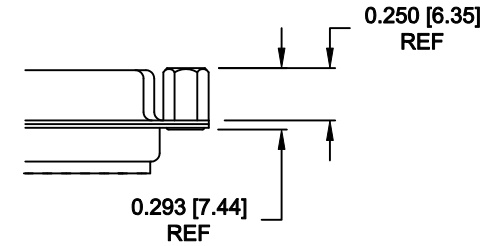
03X..... 0.250" (MATING SIDE) - CN8
