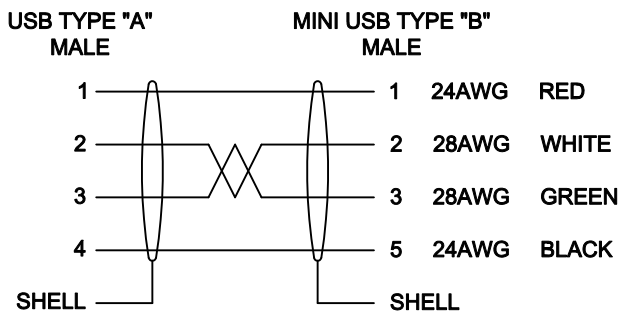
MALE-TO-MALE PINOUT
