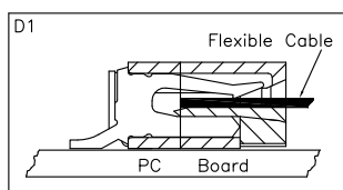
Top Contact
