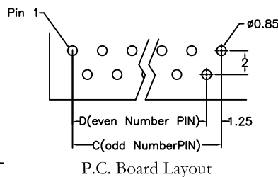
Position Dimension 3 Thru 40 A (No. of Positions X 1.25)+5.7 B (No. of Positions X 1.25)+1.4 C (No. of Positions X 1.25)-1.2 D (No. of Positions X 1.25)-1.2
