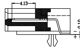
Sect B-B
