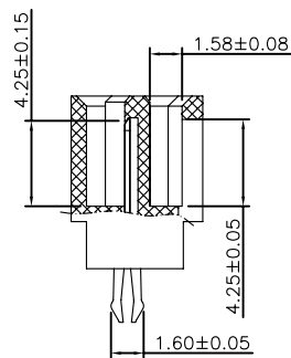
SECTION B-B
