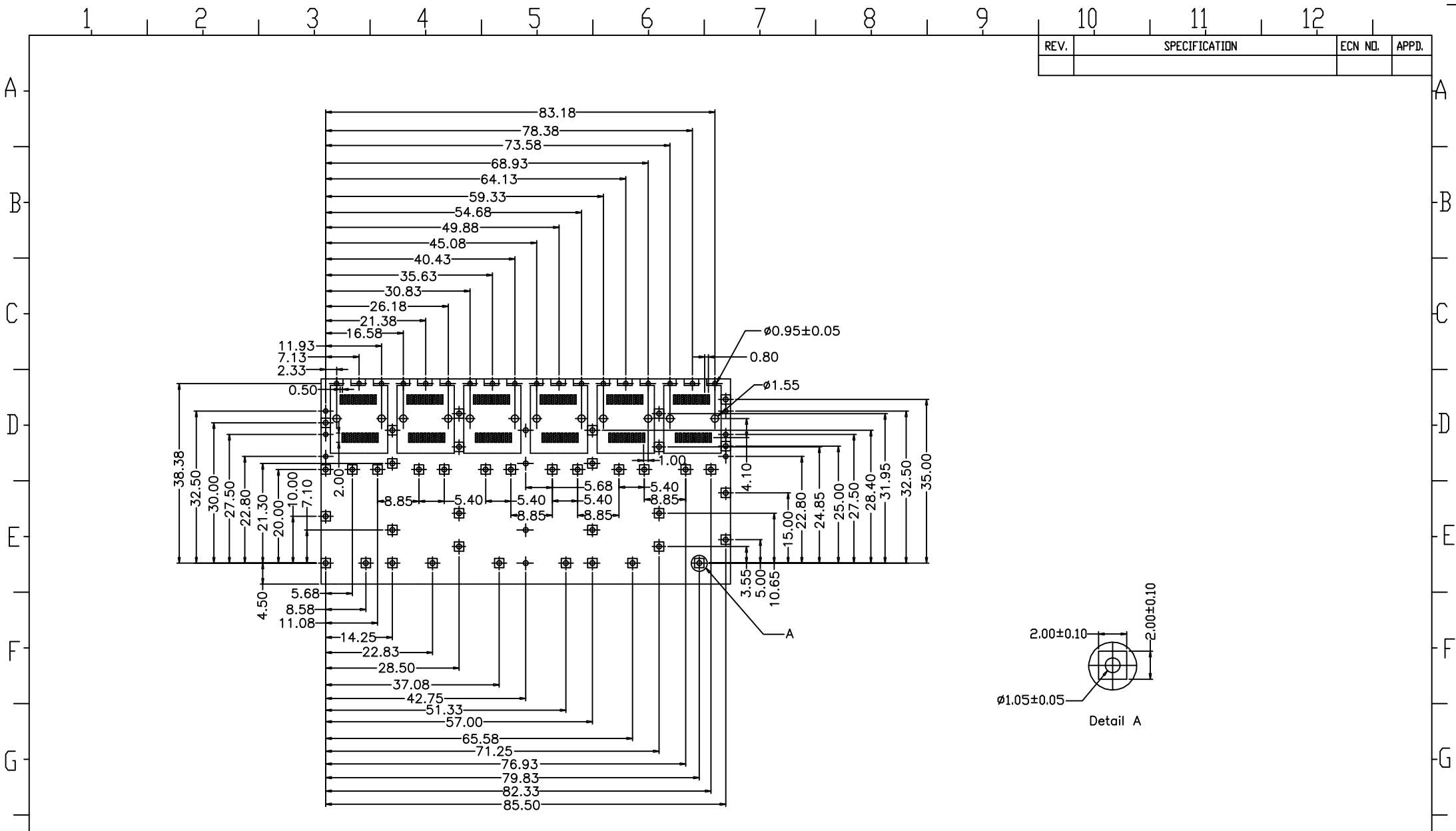
P.C.Board Layout Tolerances ±0.05
