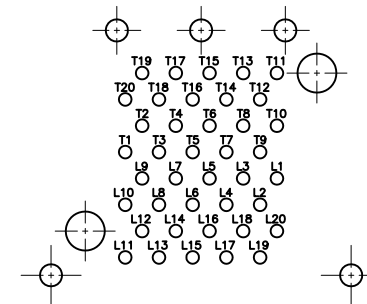
CONNETTON PINOUT DETAIL COMPONENT SIDE OF BOARD
