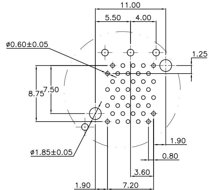
DETAIL A(SCALE 2:1)
