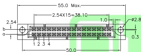
32 PIN
