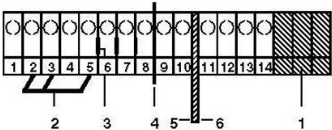
Circuit diagram
