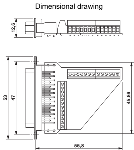
D-SUB contact insert
