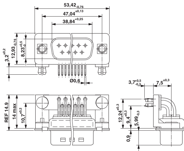
Dimensional drawing
