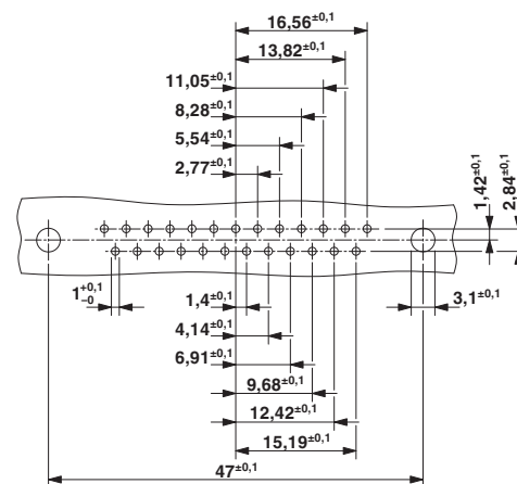
Drilling diagram
