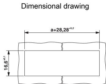
Sheet metal cutout for snap-lock device for "ST" versions
