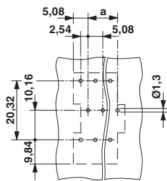
Drilling diagram
