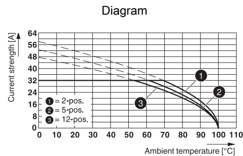
Type: IPC 5/...-ST-7,62 with IPCV 5/...-G-7,62
