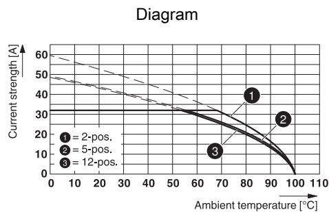
Type: IPC 5/...-ST-7,62 with IPC 5/...-G-7,62
