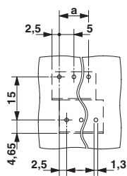
Drilling diagram
