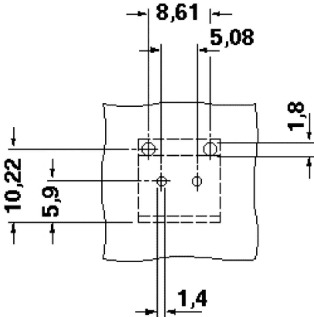
Drilling diagram
