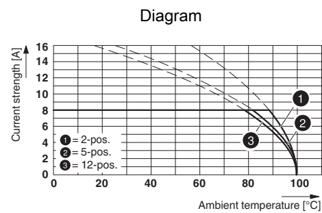
Type: MC 1,5/...-ST-5,08 with MC 1,5/...-G-5,08
