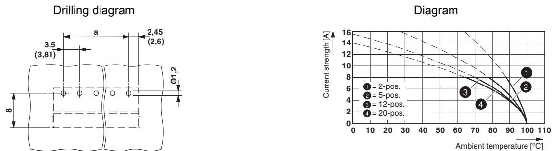
Type: FK-MCP 1,5/..-ST-3,5 with MC 1,5/..-G-3,5
