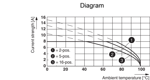
Type: MCVW 1,5/...-ST-3,5 with MC 1,5/...-G-3,5
