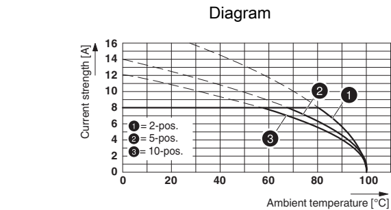
Type: TFCM 1,5/...-ST-3,5 with MC 1,5/...-G-3,5
