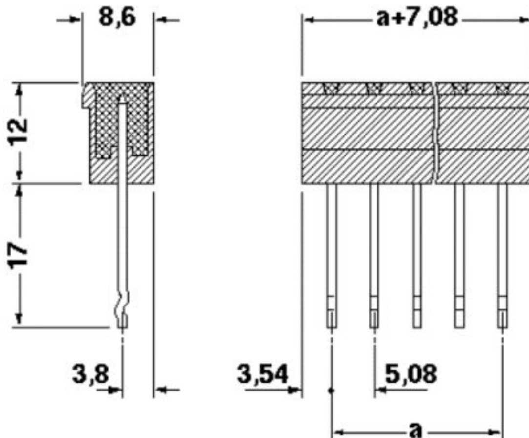
Dimensional drawing
