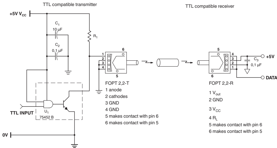
Circuit diagram
