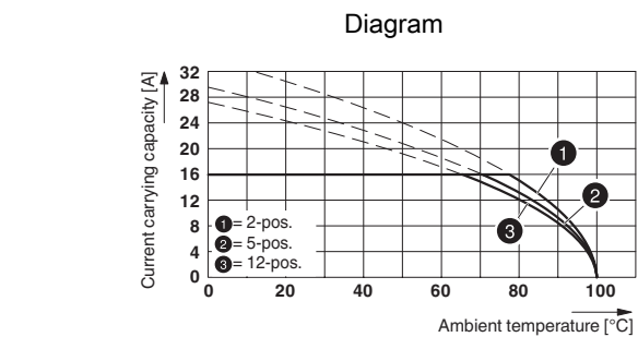
Type: MSTB 2,5 HC/...-STF with MSTBV 2,5 HC/...-GF
