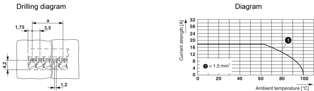
Derating diagram for 5 pins;reduction factor=1
