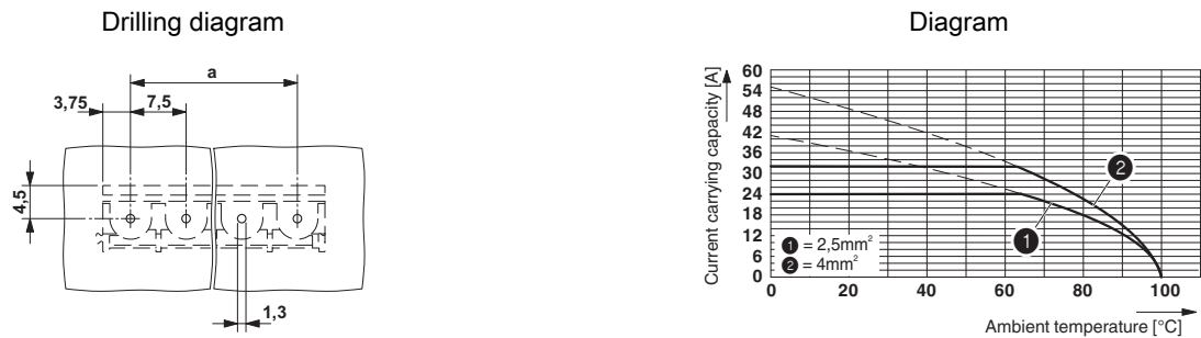
Derating diagram for 5 pins;reduction factor=1
