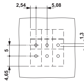
Drilling diagram
