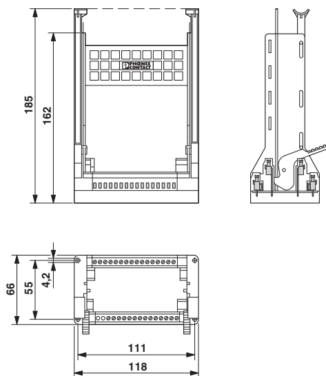
Dimensional drawing
