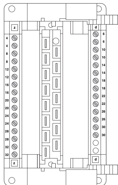
Schematic diagram
