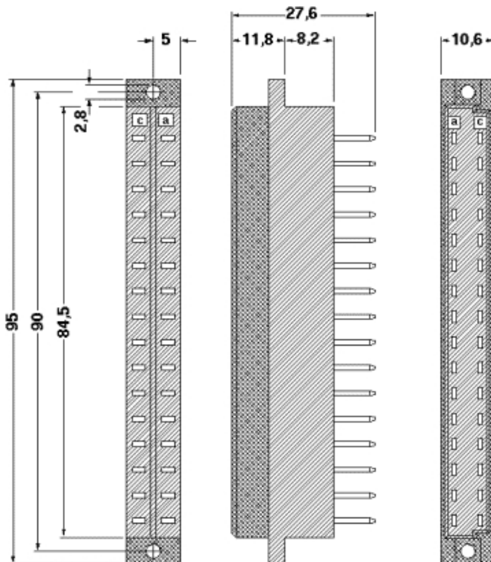
Dimensional drawing
