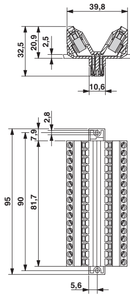
Dimensional drawing
