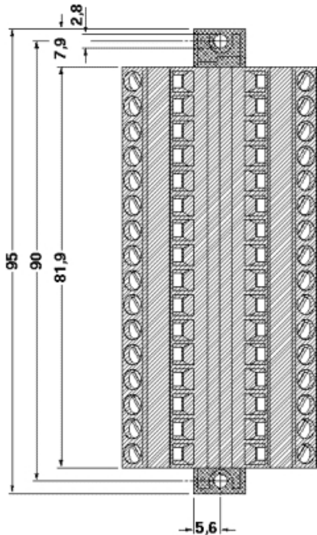
Dimensional drawing
