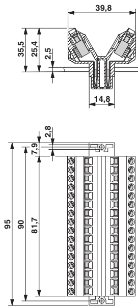
Dimensional drawing
