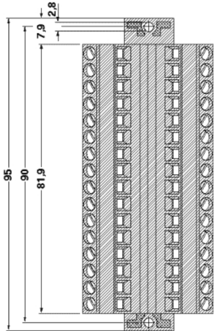
Dimensional drawing
