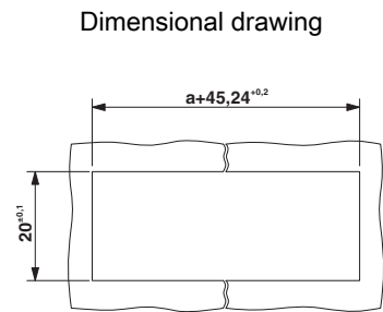
Sheet metal cutout for snap-on.
