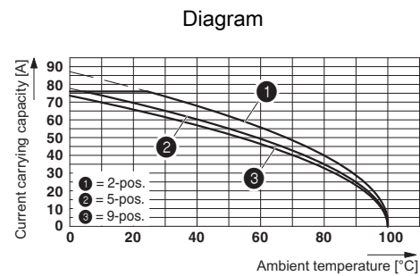
Derating curve for: IPC 16/...-ST-10.16 with DFK-IPC 16/...-ST-10.16
