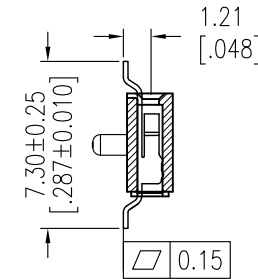
TYPE 2: WITH POST SECTION A-A
