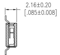
TYPE 1: W/O POST
