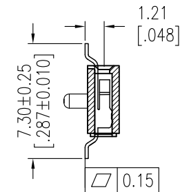
TYPE 2: WITH POST SECTION A-A
