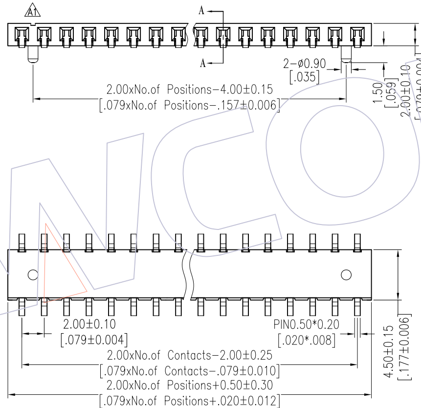
TYPE 2: WITH POST SECTION A-A
