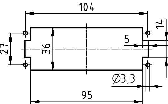
panel cut out (1:2)
