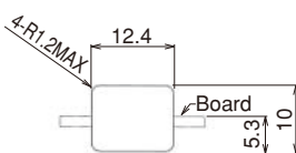
◆Recommended panel cutout dimension
