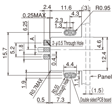
◆Recommended PCB pattern
