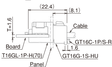
◆Mated condition
