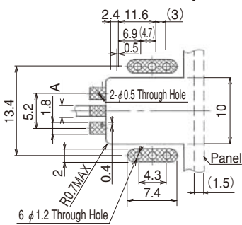
◆Recommended PCB pattern
