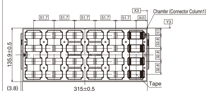
JEDEC Tray for IT3D 200 Position Receptacles
