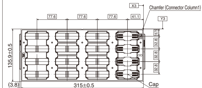
JEDEC Tray for IT3D 300 Position Receptacles
