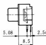
Space-saving type (RD*G)
