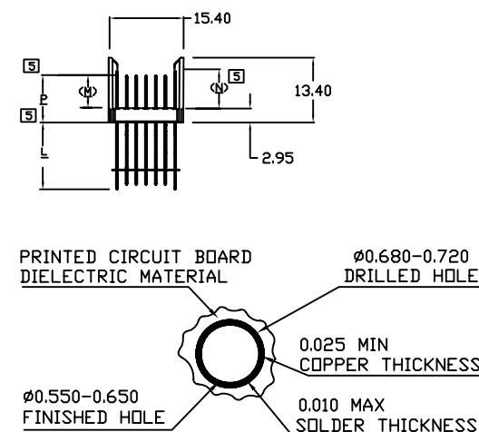
THRU HOLE PLATING SCALE 10:1
