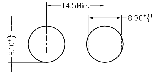
PANEL CUT-OUT
