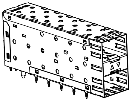
Z-824211000023X AS SHOWN WITH INNER LIGHT PIPES
