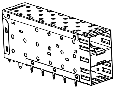
Z-824211000003X AS SHOWN WITHOUT LIGHT PIPE
