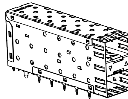
Z-824211000033X AS SHOWN WITH OUTER LIGHT PIPES
