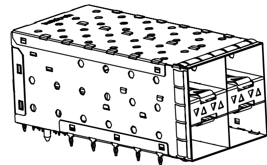
Z-824221000011X AS SHOWN WITH INNER & OUTER LIGHT PIPES
