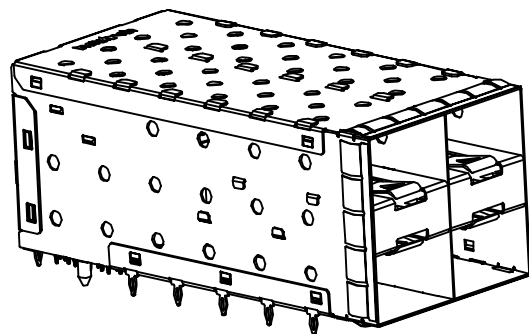
Z-824221000001X AS SHOWN WITHOUT LIGHT PIPE
