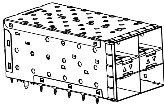
Z-824221000021X AS SHOWN WITH INNER LIGHT PIPES
