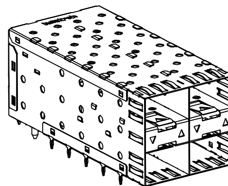
Z-824221000033X AS SHOWN WITH OUTER LIGHT PIPES
