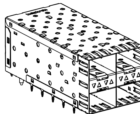
Z-824221000013X AS SHOWN WITH INNER & OUTER LIGHT PIPES
