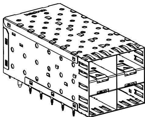
Z-824221000003X AS SHOWN WITHOUT LIGHT PIPE
