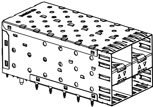
Z-824221000120X AS SHOWN WITH INNER LIGHT PIPES
