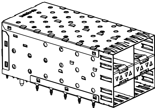
Z-824221000110X AS SHOWN WITH INNER & OUTER LIGHT PIPES
