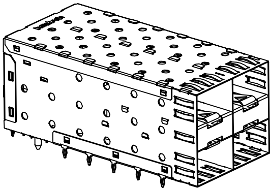
Z-824221000100X AS SHOWN WITHOUT LIGHT PIPE
