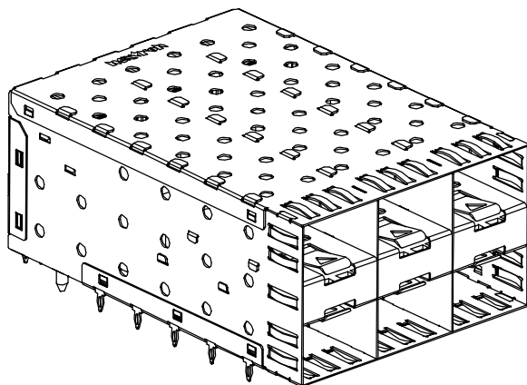
Z-824231000003X AS SHOWN WITHOUT LIGHT PIPE
