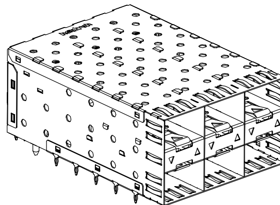
Z-824231000033X AS SHOWN WITH OUTER LIGHT PIPES
