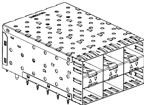
Z-824231000023X AS SHOWN WITH INNER LIGHT PIPES
