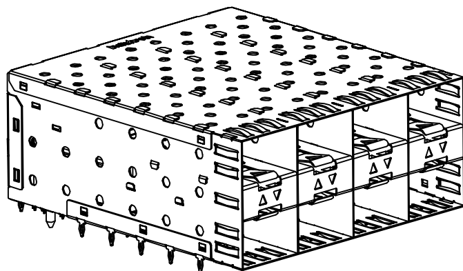
Z-824241000120X AS SHOWN WITH INNER LIGHT PIPES
