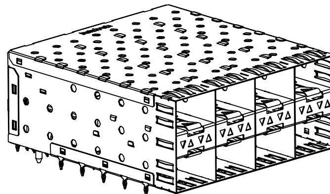
Z-824241000110X AS SHOWN WITH INNER & OUTER LIGHT PIPES
