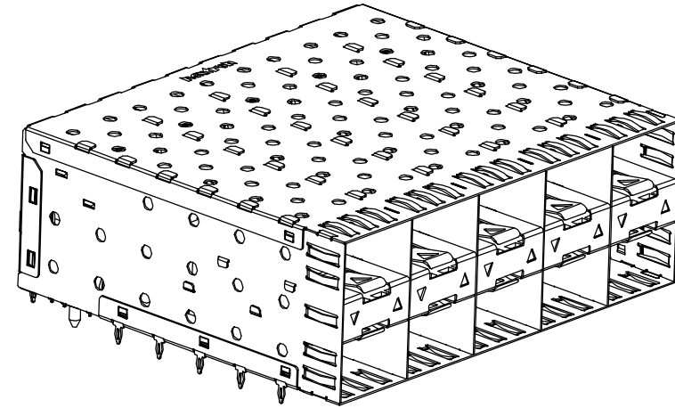
Z-824251000030X AS SHOWN WITH OUTER LIGHT PIPES
