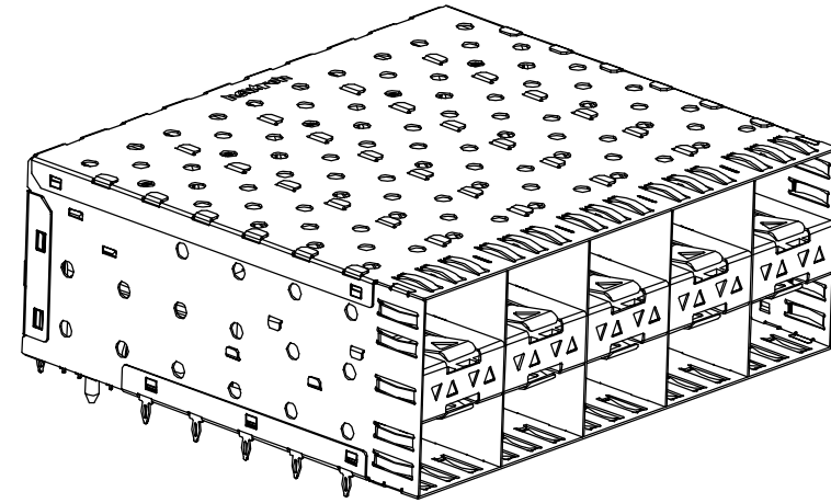
Z-824251000010X AS SHOWN WITH INNER & OUTER LIGHT PIPES
