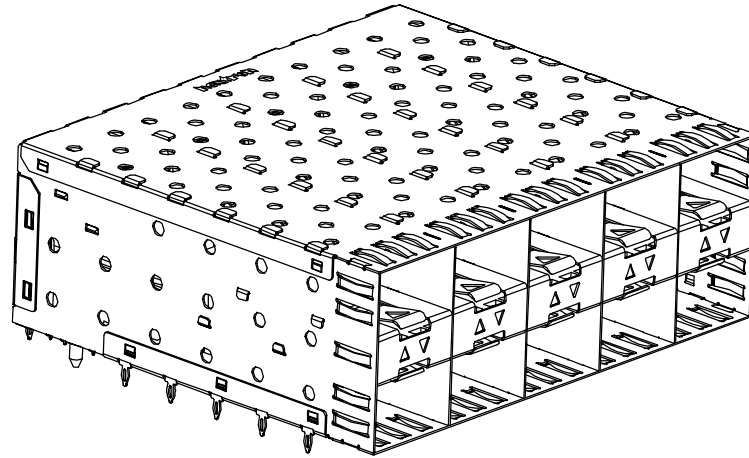
Z-824251000020X AS SHOWN WITH INNER LIGHT PIPES
