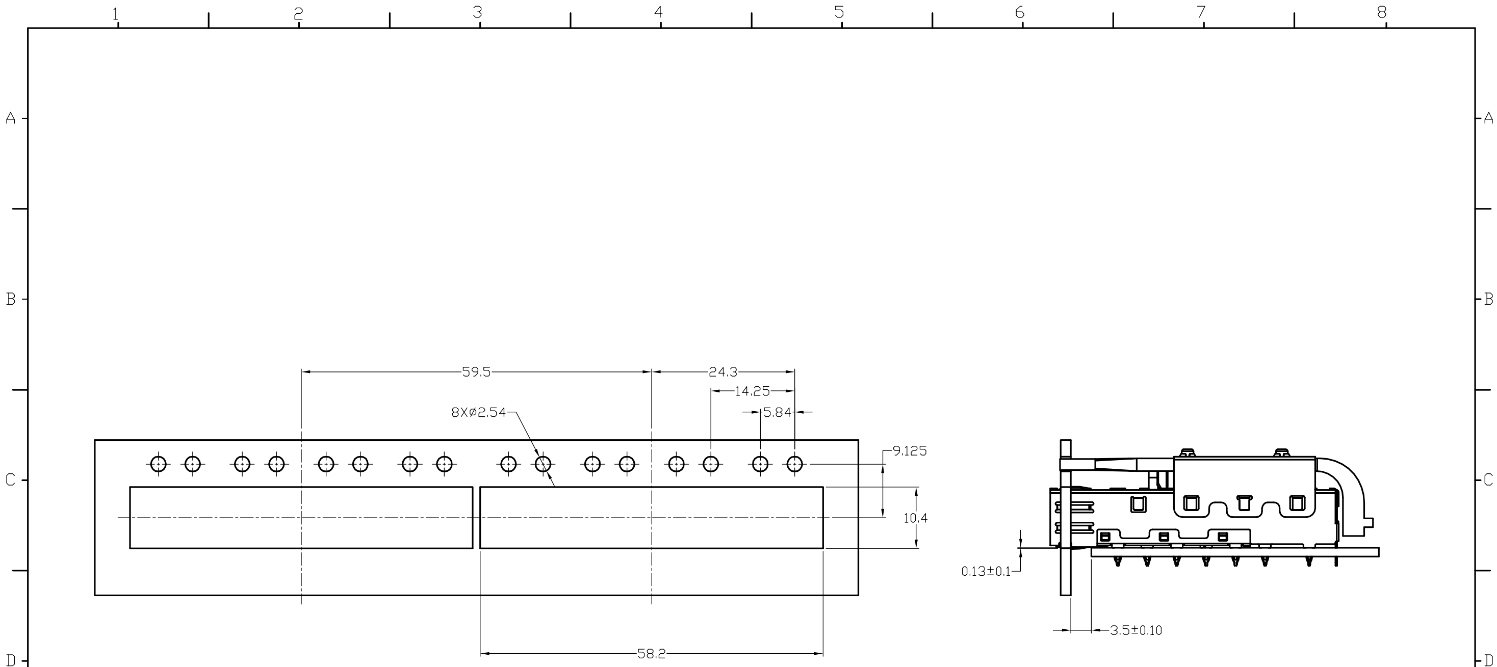
RECOMMENDED BEZEL CUT-OUT AND BOARD POSITION DIMENSIONS FOR SINGLE SIDE MOUNTING
